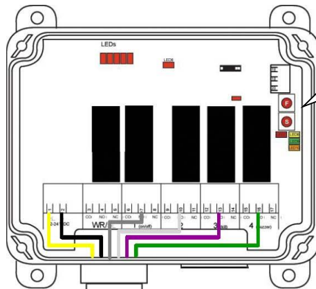
Receiver (Part # 3239)
